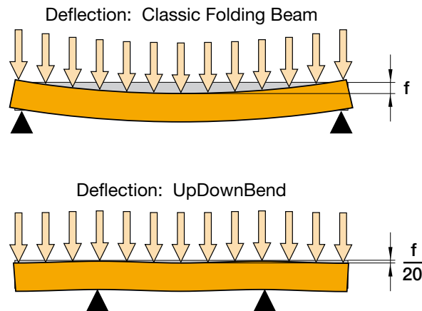
The beam-in-beam concept supersedes a crowning system
