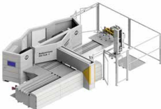
Multibend-Center with manual part unloading via finished part buffer or automatically by intelligent robot. Rotation station for finished parts. Provision of the pallets by U-shaped pallet station.
