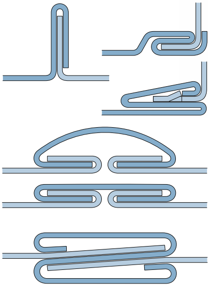
Standing seam, Pittsburgh seam, Snaplock seam, and „S“ seam
