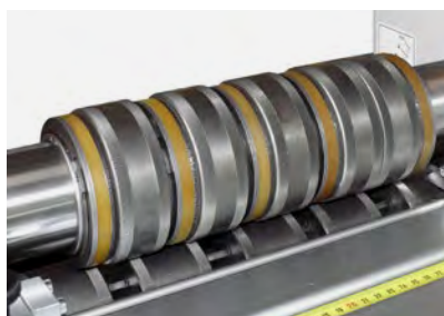
Rolls for standing seam and snap-lock seam.
