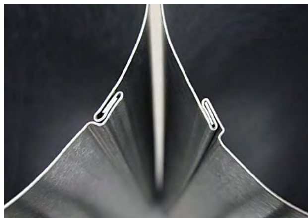
Quick changeover from inside to outside seams.
