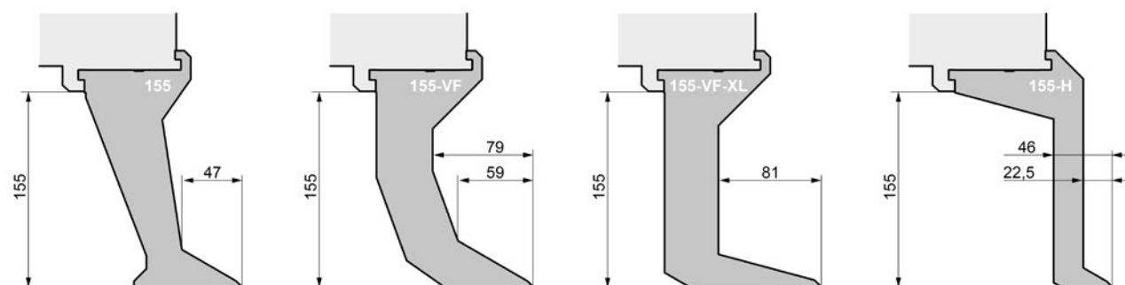
Clearance options using upper beam tools with 155mm in height as an example.
